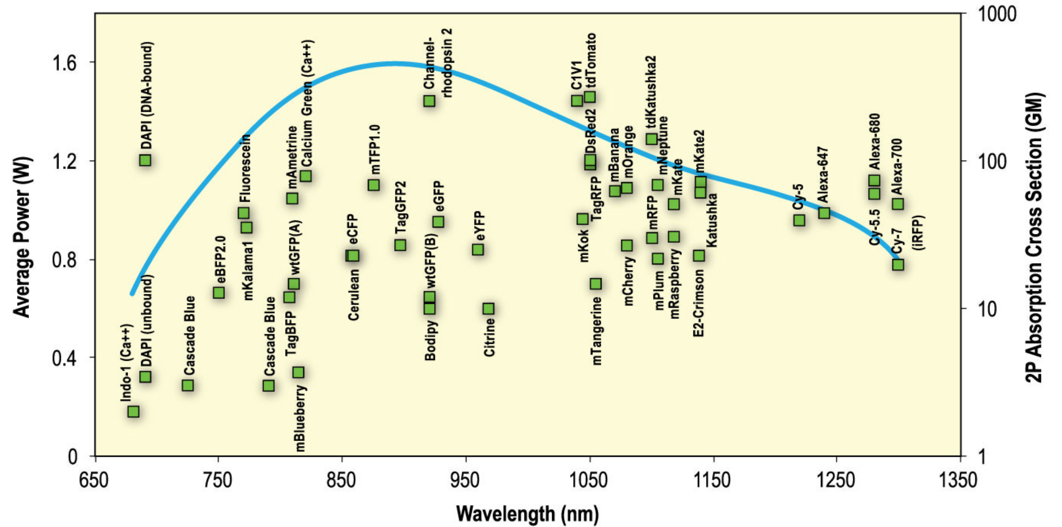
InSight DS+ Two-Photon Excitation Curve
